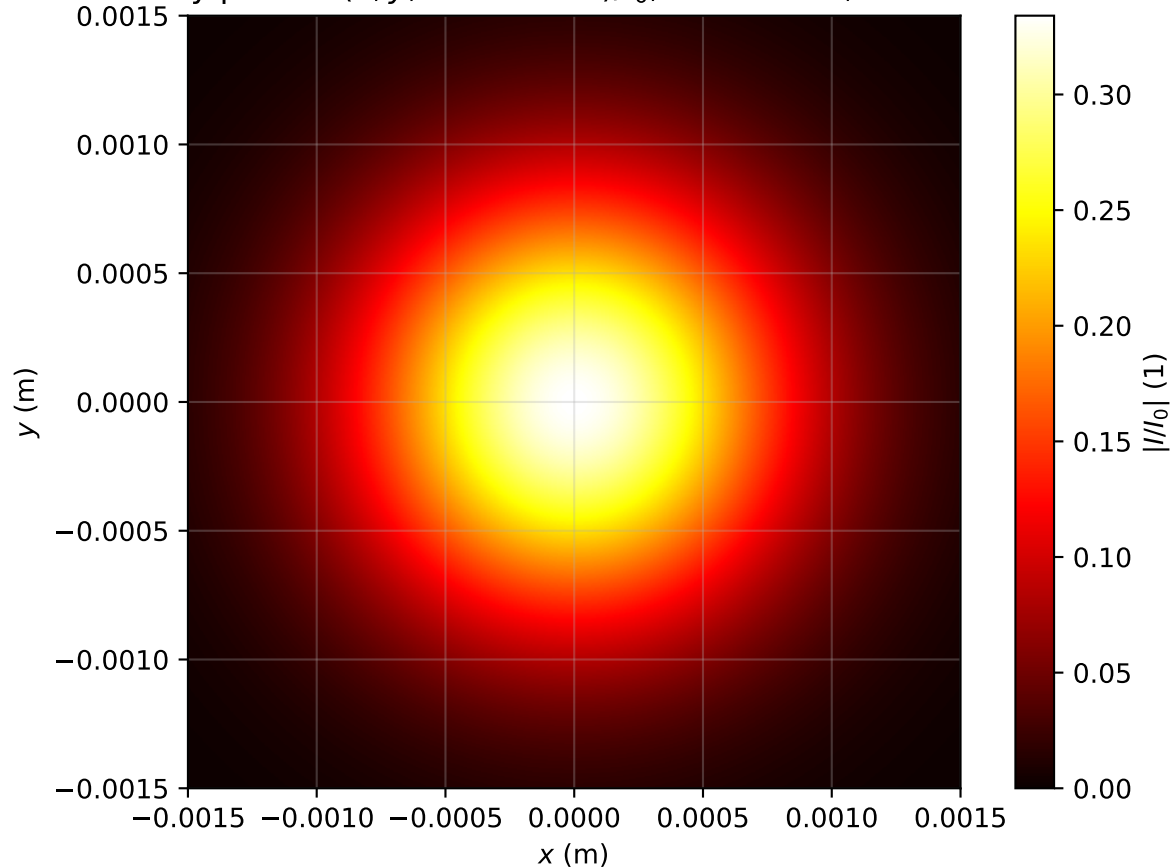
Intensity profile I(x, y, z = 3.264m)/I_0 , P_{in}=0.2P_{cr} , artificial time
